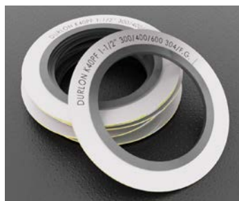
Durlon® Kammprofile Serrated Flat Metal Gaskets Grooved metal gasket with covering layers
